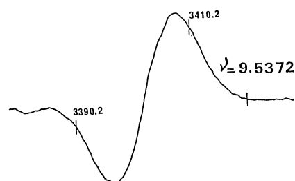
Fig. 4. ESR spectrum of cis -stilbene radical cation ( cis -3 + ) in \text{CFCl}_3 matrix at 140 K.
