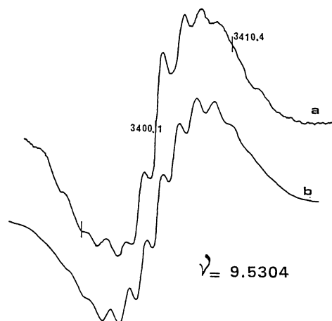
Fig. 3. a) Experimental ESR spectrum of trans -stilbene radical cation ( trans -3 + ) in \text{CFCl}_3 matrix at 140 K. b) Simulated spectrum with parameters in Table 1.
